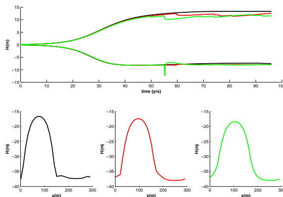
Figure 8. Sand wave growth (top) and shape (bottom) with a wave height of 0 m (left), 5.0m (middle) and 7.0 m (right), all for a water depth of 30 m and a depth averaged current of 0.5 m/s at maximal tide.
