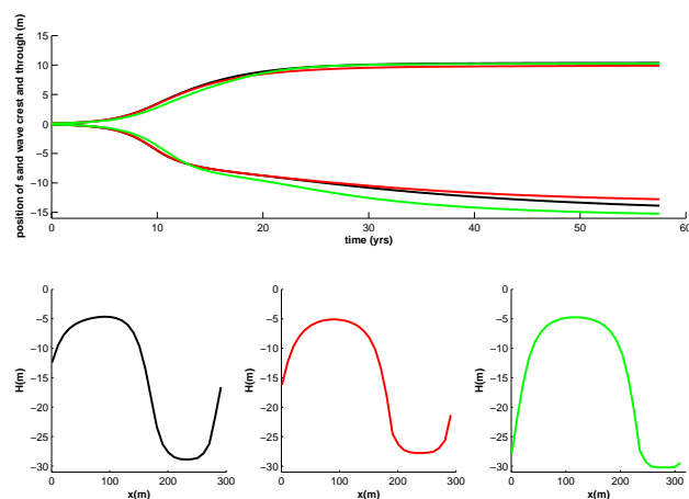
Figure 6. Sand wave growth (top) and shape (bottom) with a wave height and period of 0.5m and 4 s (left) , 1.0m and 7 s (middle) and 2 m and 12 s (right).
